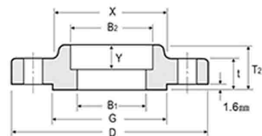
SOCKET WELDING
