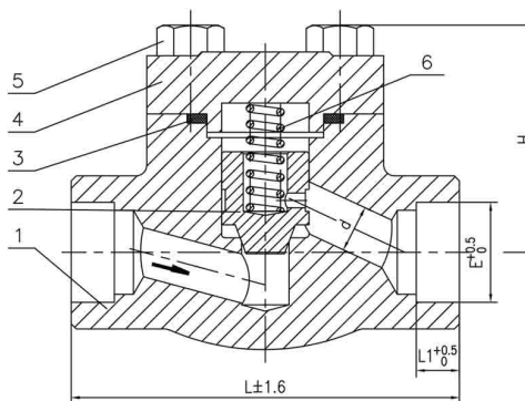
Socket Welding Type
