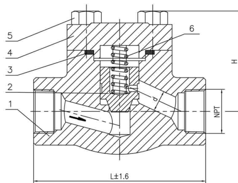
Screw End Type (NPT)
